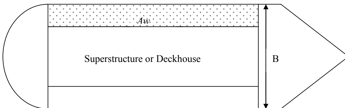
Figure 2.2 FP_{REQ} = \frac{0.28 \times A_w}{B}
